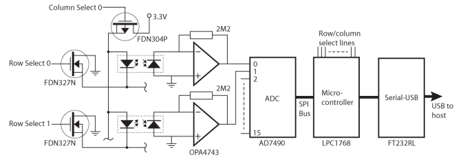
Figure 4. Sensor circuit diagram.
