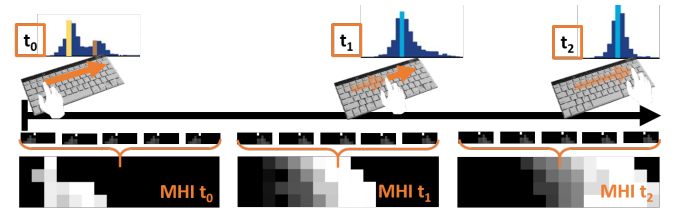
Figure 11. Generating a motion history images. Each MHI contains 160 frames of history. All frames t_1 to t_2 are labeled as a specific gesture in the training data. At test time each pixel in the MHI is classified. All MHIs within t_1 - t_2 range will be labeled as the corresponding class.
