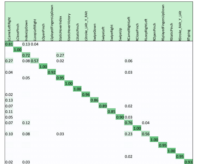
Figure 12. Confusion matrix for all 22 recognized gestures, test data recorded from 11 participants. Results from our forest-based classifier; mean success rate 88.9%.
