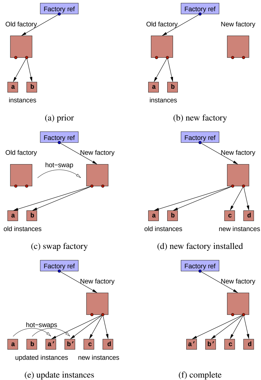
Figure 4.9: Phases in the dynamic update of a multiple-instance object without adaptors or laziness: (a) prior to update the old factory is maintaining instances of a class; (b) instantiate a new factory for the updated class; (c) hot-swap the factory with its replacement (transferring the set of managed instances, and transparently swinging the factory reference); (d) after the hot-swap, new instantiations are handled by the updated factory code (thus creating objects of the new type); (e) update old instances by hot swapping each to an updated replacement; (f) the update is complete.
