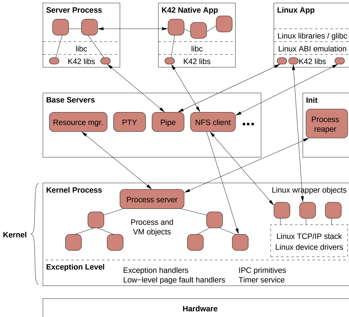
Figure 4.1: Structural overview of K42. Arrows indicate possible protected procedure calls between objects in different processes.
