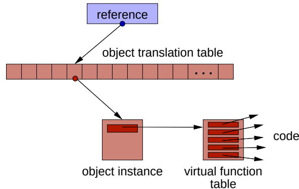
Figure 4.4: Clustered object indirection through object translation table
