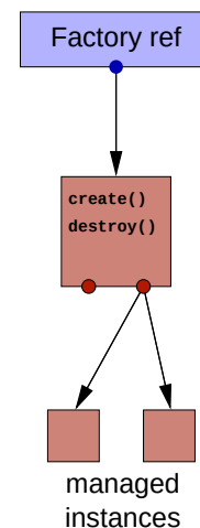
Figure 4.7: Factory object
