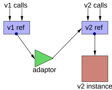
Figure 4.8: Adaptor object
