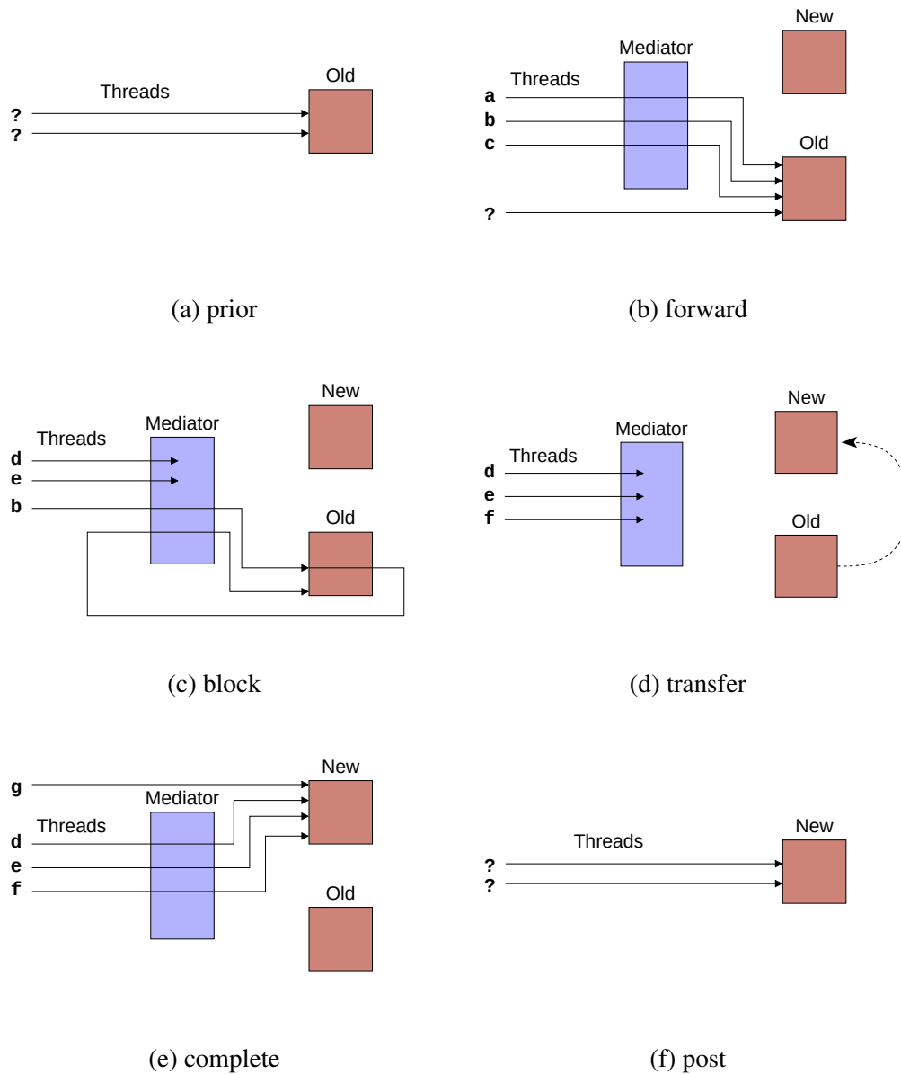
Figure 4.5: Phases in an object hot-swap: (a) prior to the swap threads invoke an object directly; (b) a mediator object is interposed, forwarding new calls to the object; (c) once all calls are tracked, the mediator blocks incoming calls and waits for the existing ones to finish; (d) when the object is quiescent, state is transferred to its replacement; (e) the mediator forwards blocked calls to the new object; (f) the old object and mediator are destroyed. Reproduced from Appavoo et al. [AHS + 02].
