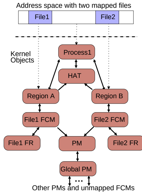
Figure 4.2: Virtual memory system object hierarchy. Reproduced from Appavoo [App05].
