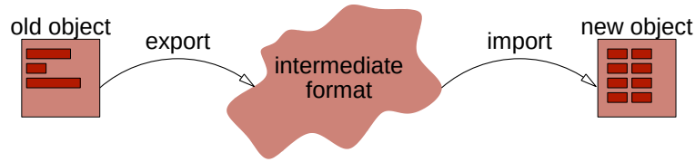
Figure 4.6: State transfer
