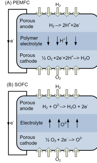
Figure 1: Schematics of (A) PEMFC and (B) SOFC.
