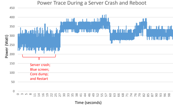
Figure 6: The Power trace from a server crash and reboot sequence under 48V DC.
