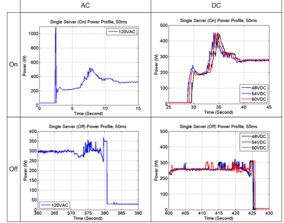
Figure 10: Single server power-on and power-off characterization.
