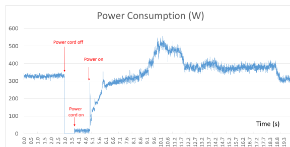
Figure 2: The power trace from powering down and starting up a server under 48V DC.
