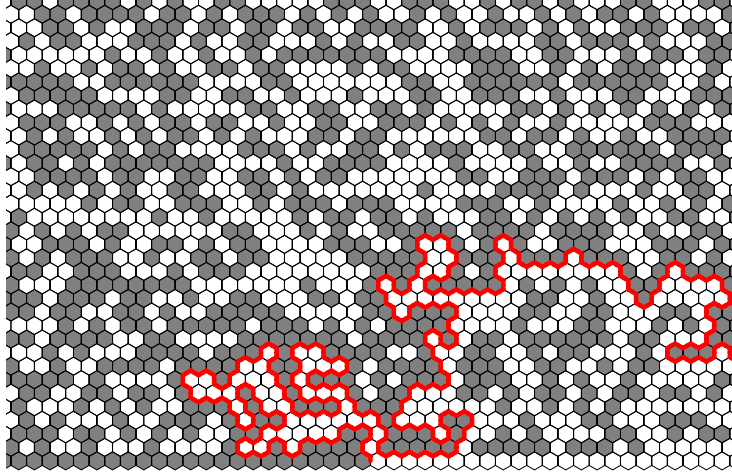
Figure 2: The percolation boundary path
