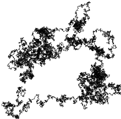
Figure 1: Simulation of a planar Brownian path
