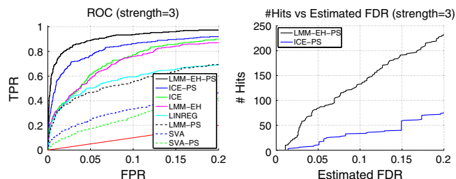
Fig. 4. Power curves for synthetic mouse data. The left plot shows the ROC curve, where our model LMM-EH-PS achieved maximum power. The red line denotes what random guessing would have achieved. The right plot illustrates how the best ICE-based model (ICE-PS), which yielded deflated p -values, penalized itself because of its overly conservative estimated FDR.
