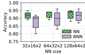
Figure 13: Box plot of the accuracies for the predicted queues in the network tomography use case. BNNs makes our approach practical while trading just a tiny amount of accuracy with respect to non-binarized NNs.
