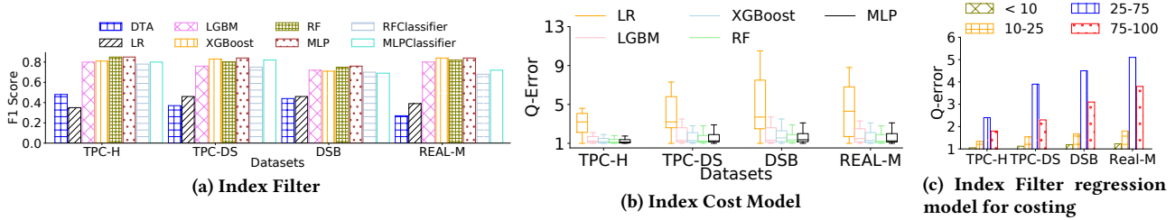
Figure 8: a) and b) evaluate the effectiveness of different ML algorithms for Index Filter and Index Cost Model. In c), we evaluate the effectiveness of using Index Filter regression model for costing. The (query, configuration) pairs are grouped based on actual improvements, e.g., the bar < 10 represents a group of (query, configuration) pairs where actual improvement is < 10\% .
