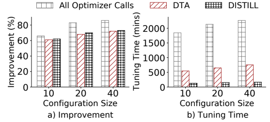
Figure 1: Impact of DISTILL on performance improvement and tuning time on TPC-DS workload consisting of 910 queries
