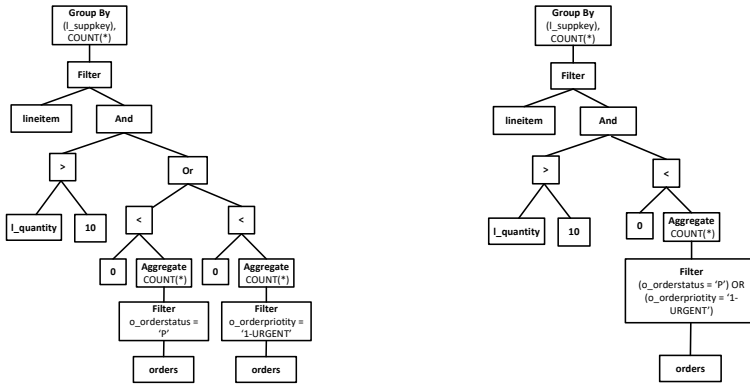
(a) Original logical expression with two correlated subqueries
