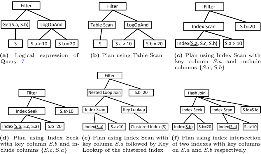
Figure 4.1: Plans using different access methods to execute Query 7
